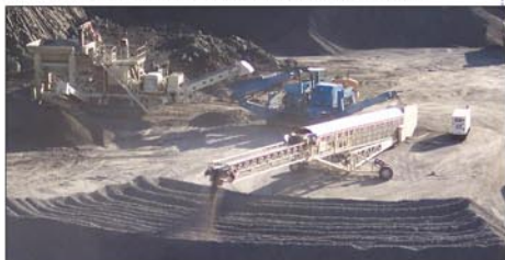
Radial Telescopic Conveyor automatic windrow Stockpiling 'In Specification' aggregate material from a primary and secondary Crusher - 600TPH
